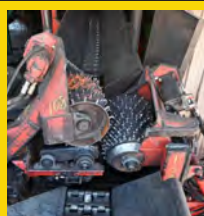
Morbark Debarker
