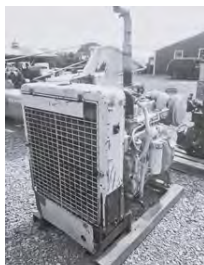
Cat 3304 , 115 HP, Radiator Thru Flywheel, 3000 Hrs, $4,500
