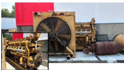
Kato Engineering 1030 AC generator / 16 Cylinder Cat D399 Diesel Motor Generator Set Generator Capacity: 1030 kW continuous duty. Voltage: 346/600V or 480V, 3-phase. Cat D299 Diesel Motor: 1,250 HP at 1,200 RPM Price: $35,000.00 (1 Available)
